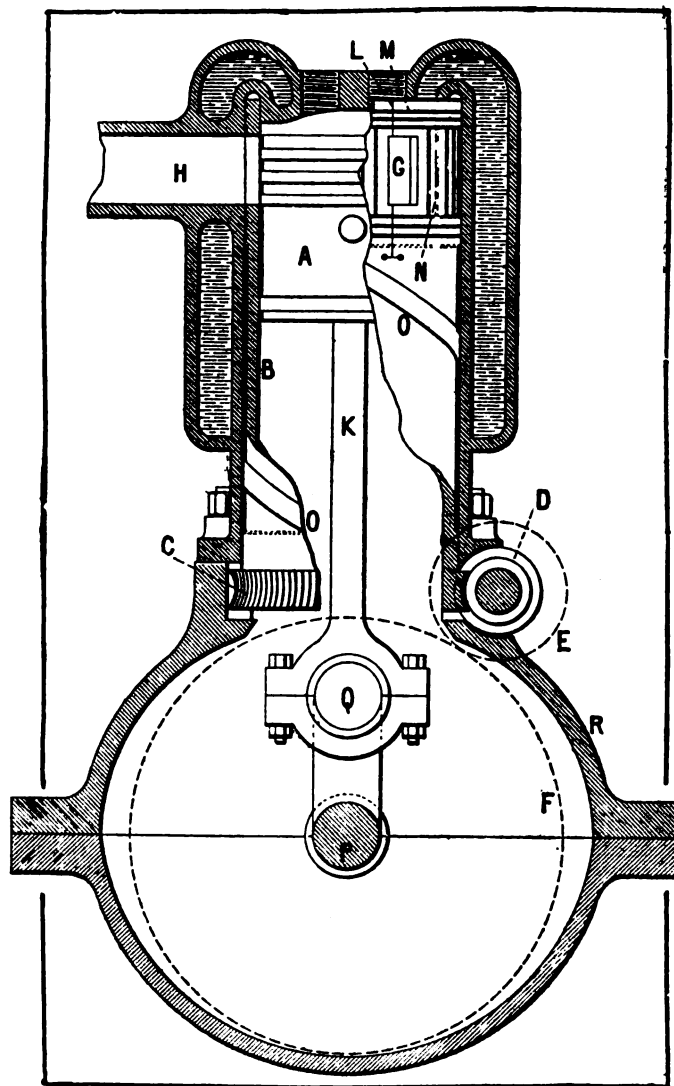
Section Through Ledru Motor Showing Sleeve.
